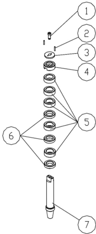
1-1/4" Spindle
