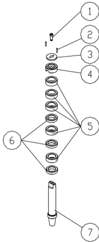
1-1/4" Spindle
