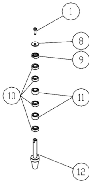
3/4" Spindle
